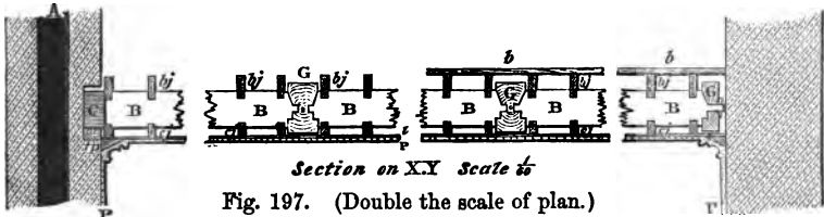
Fig. 197. (Double the scale of plan.)
